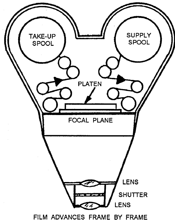
Figure 6-16.—Framing camera.
